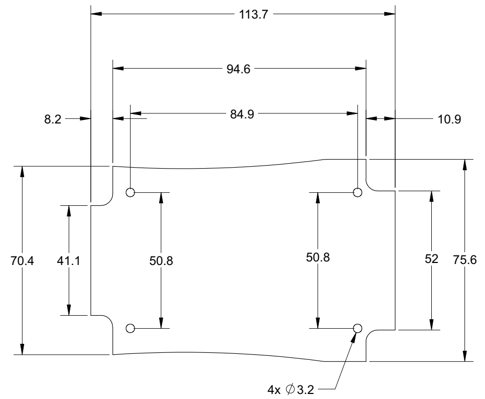
BOTTOM PCB MOCK-UP
